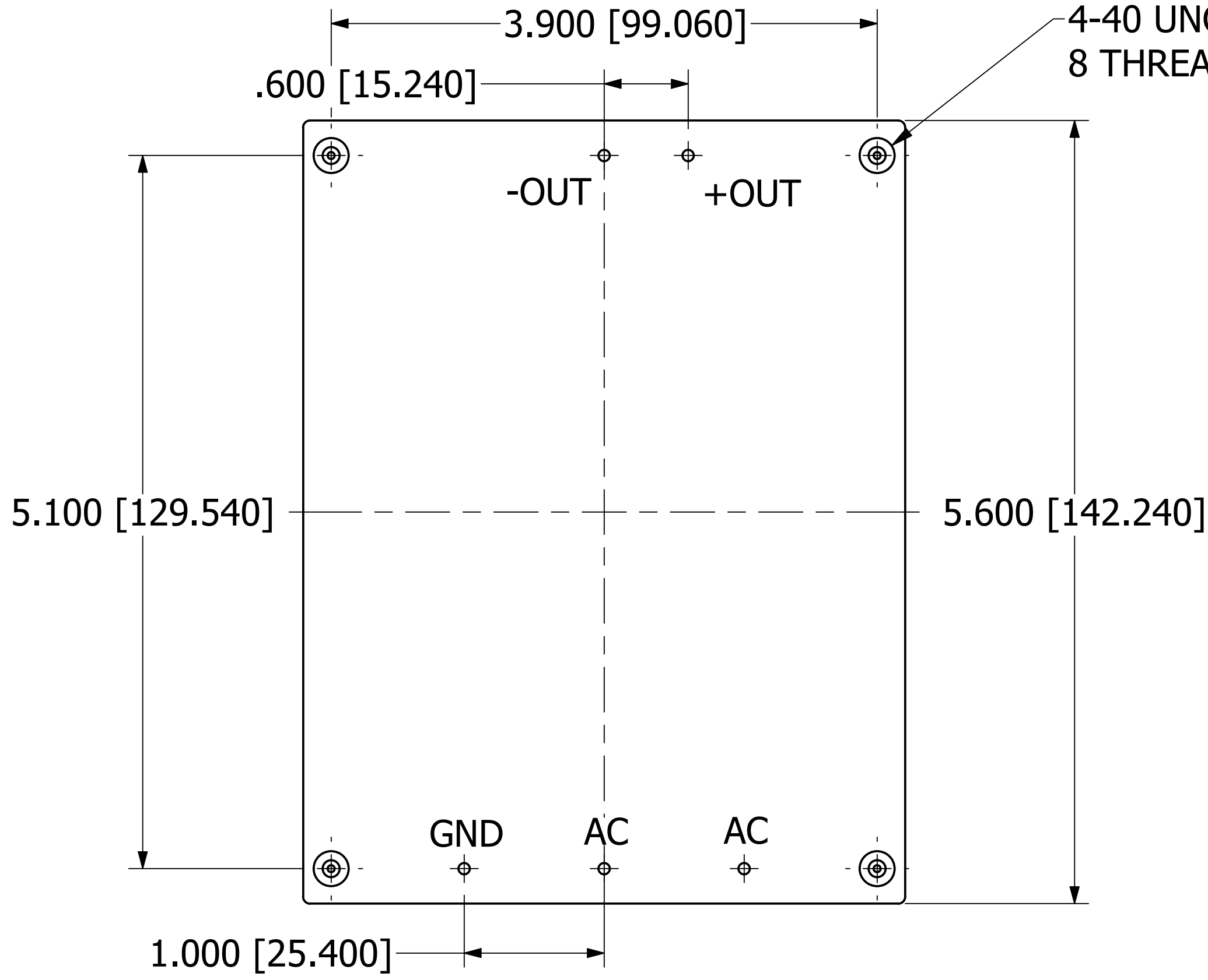
BOTTOM VIEW
